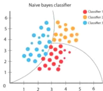
Figure 3: Naive Bayes
