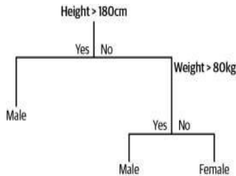
Figure 7: Decision Trees
