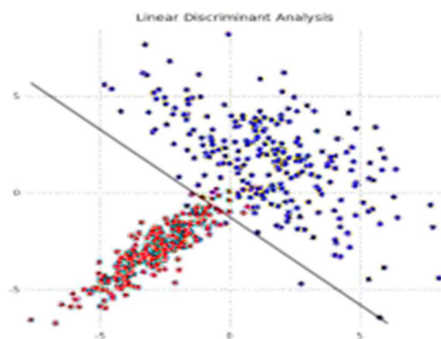
Figure 5: Discriminant Analysis
