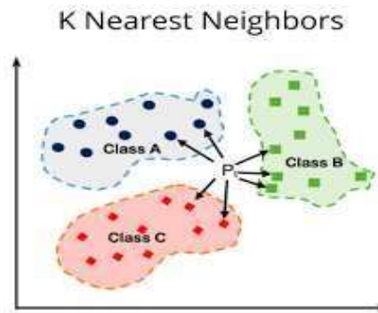
Figure 4: K-Nearest Neighbor
