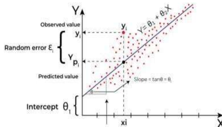
Figure 6: Linear Regression
