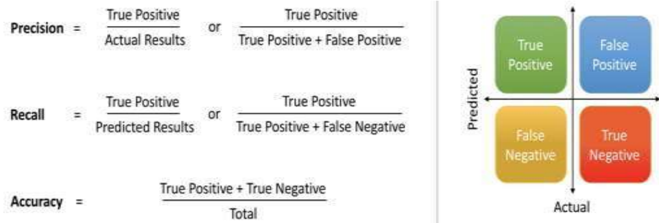
Figure 8: Evaluation of Model Performance
