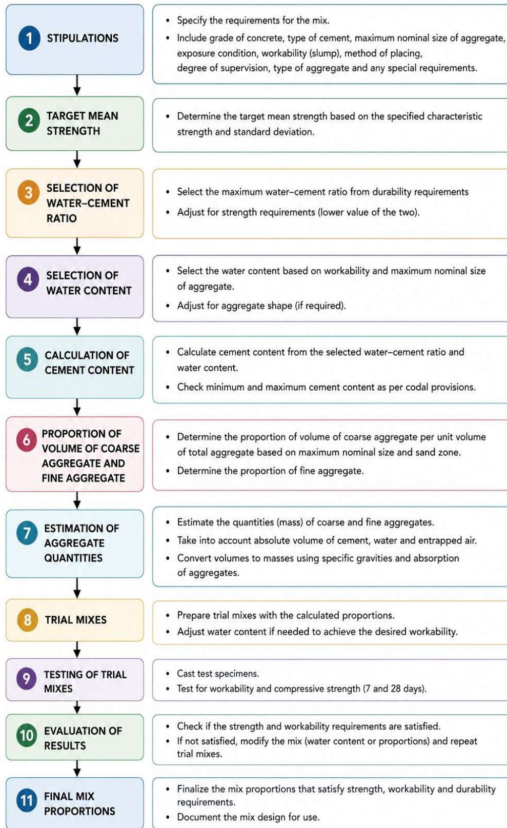
Fig. 3.1 Typical mix design flow chart
